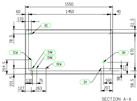
PIPES POSITIONS FOR FRONTAL AIR SUCTION VERSION
