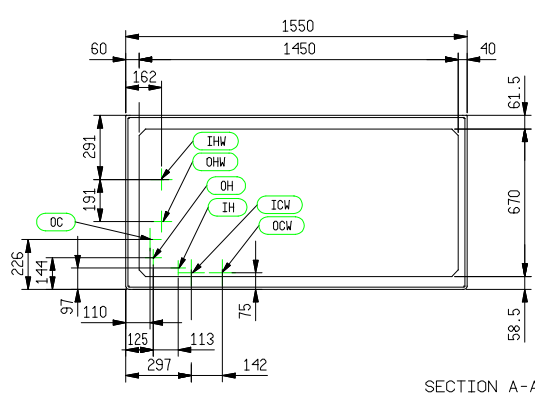
PIPES POSITIONS FOR REAR/BOTTOM AIR SUCTION VERSION
