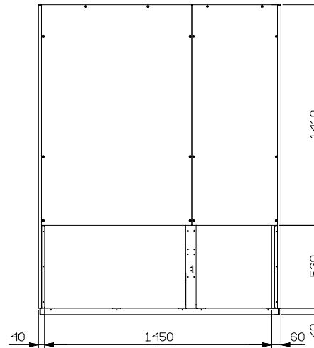
OPTION REAR AIR INTAKE ONLY WITH EC Radial Fan
